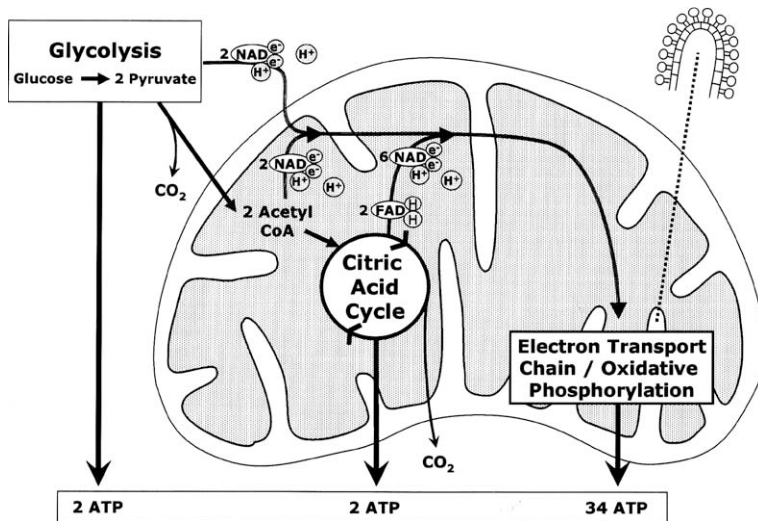
Fig. 4. Localization of the three major operations of cellular respiration in parts of the cell: glycolysis in the cytoplasm, the citric acid (krebs) cycle in the mitochondrial matrix, and the electron transport chain and oxidative phosphorylation in the cristae of the mitochondrion. Also shown is the energy yield from each operation (number of molecules of ATP synthesized from ADP).
