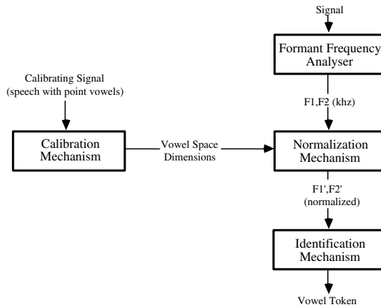
Fig. 2. The Gerstman vowel normalization model.
